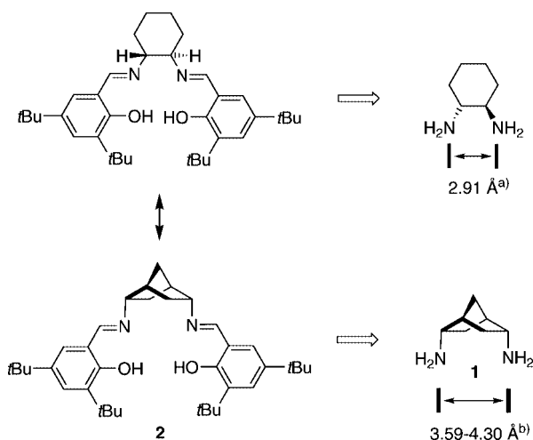
Figure 1. Salen ligands derived from trans -1,2-diaminocyclohexane and DIANANE, and the corresponding N–N distances. a) N–N distance in the ligand derived from 3,5-di- tert -butylsalicylic aldehyde [40] . b) N–N distances in various differently substituted salen ligands [39,41]
