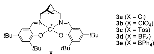
Figure 2. DIANANE–Cr III –salen complexes 3a–e bearing different counteranions.
