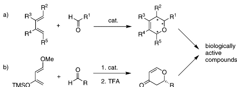
Scheme 1. HDA reaction of dienes with aldehydes (equation a) and of Danishefsky's diene with aldehydes (equation b).
